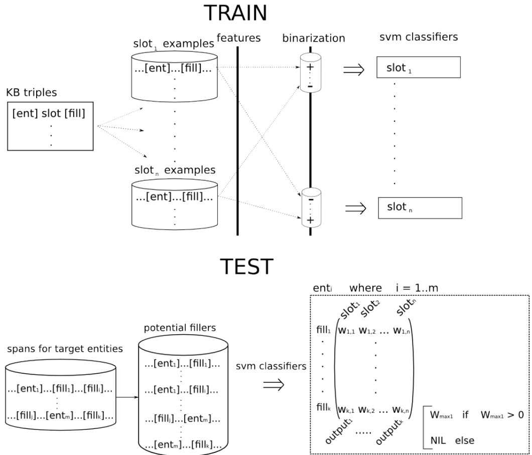
Fig. 1. The architecture of the slot filling system. TRAIN: Extraction of KB triples, which are used to acquire training examples for each slot ( 1..n slots) from the document base, followed by featurization and binarization. We finally train n classifiers, one per slot. TEST: examples containing mentions to the target entities ( m entities) are retrieved from the document base ( m target entities). Potential fillers are identified, and then each example containing one entity-filler is classified, obtaining a weighted prediction for each slot. Predictions are collated and the result returned.
